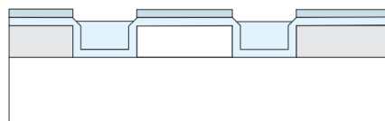
(c) Fill Trench with Dielectric
